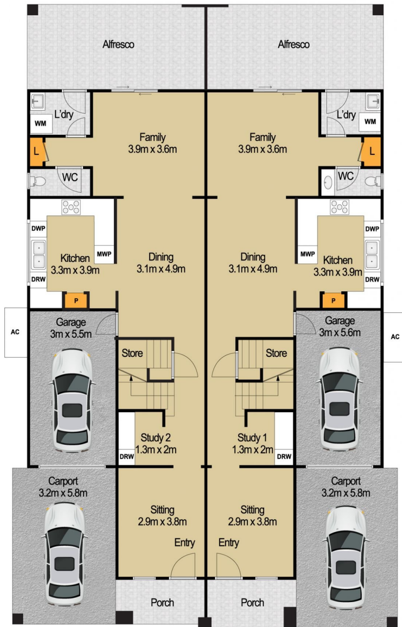
GROUND FLOOR
