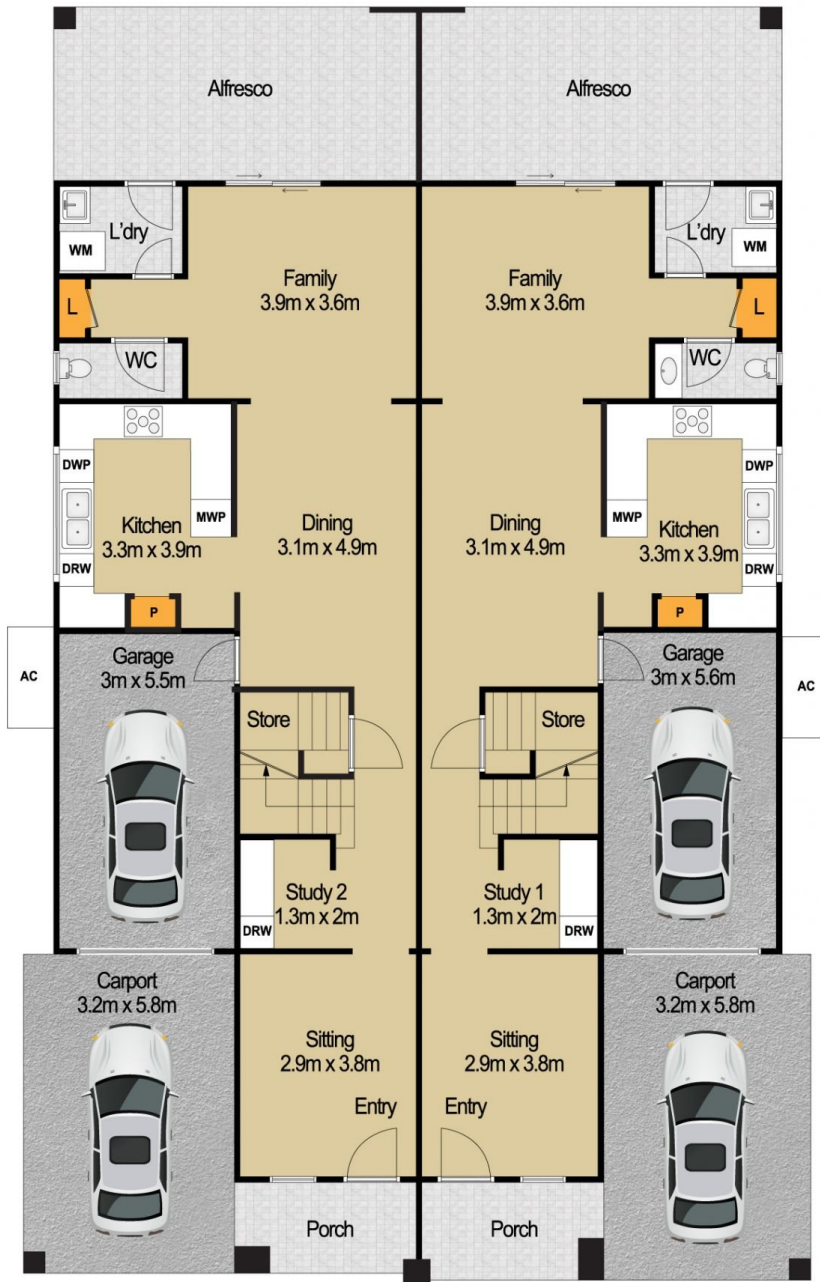
GROUND FLOOR
